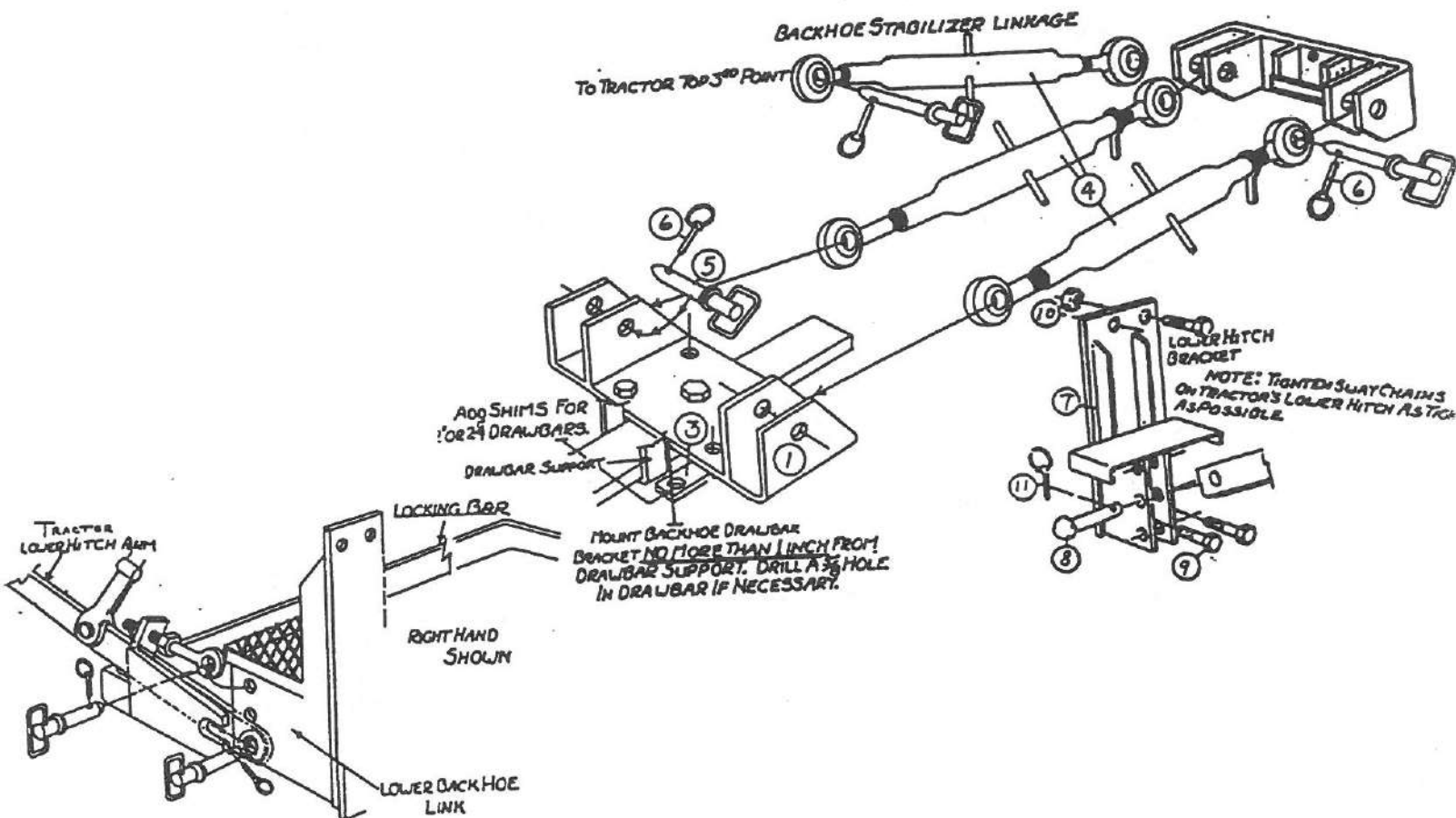
OPTIONAL - LOCKING BAR MOUNT KIT-B-851 SHOWN
