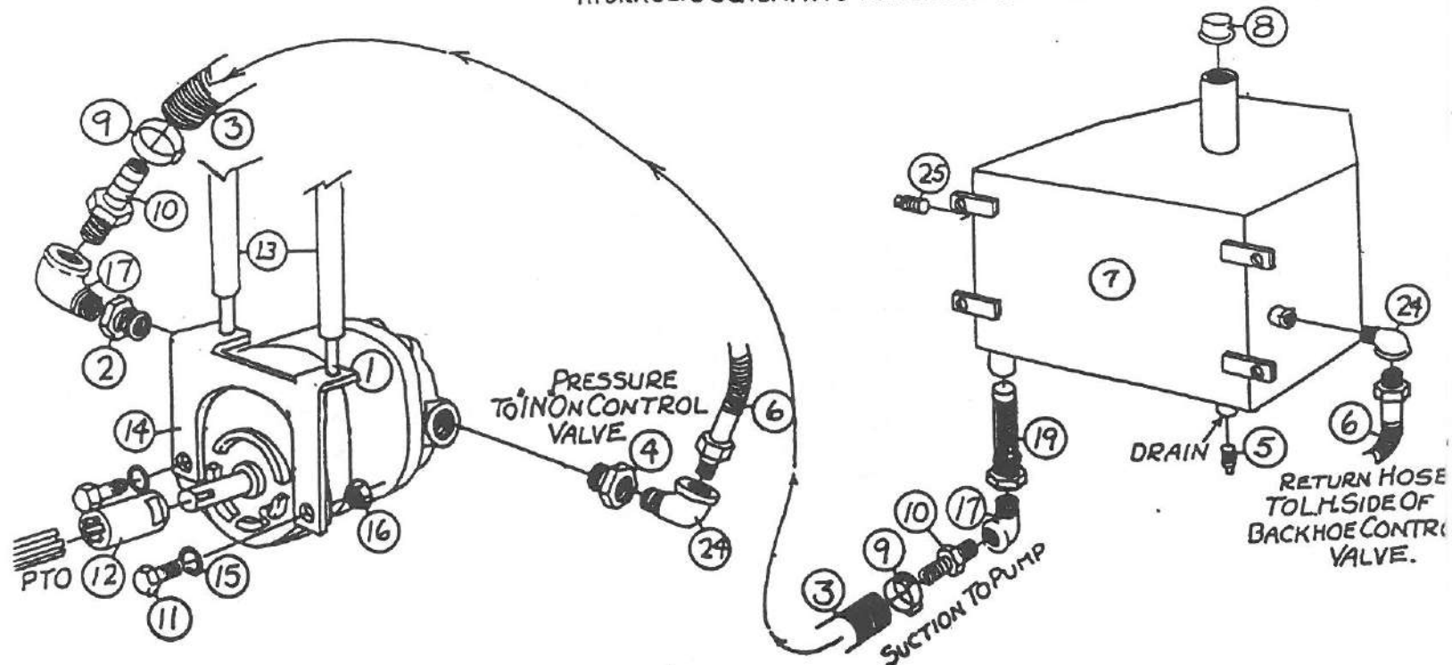
HYDRAULIC SCHEMATIC FOR B51 BACKHOE
