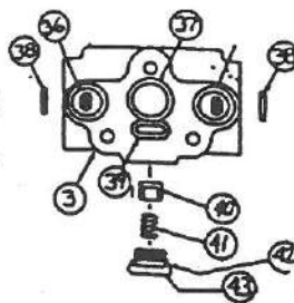
DIRECT RELIEF VALVE CARTRIDGE W/EXTERNAL ADJUSTMENT CODE LETTER 'F' 785056
