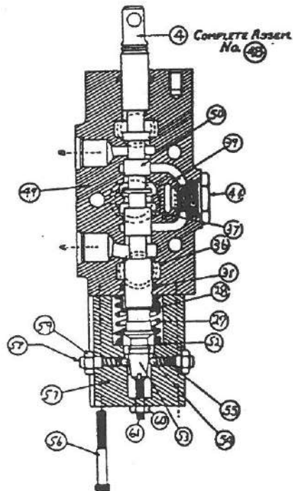
DIRECT RELIEF VALVE CARTRIDGE W/EXTERNAL ADJUSTMENT CODE LETTER 'F' 785056
