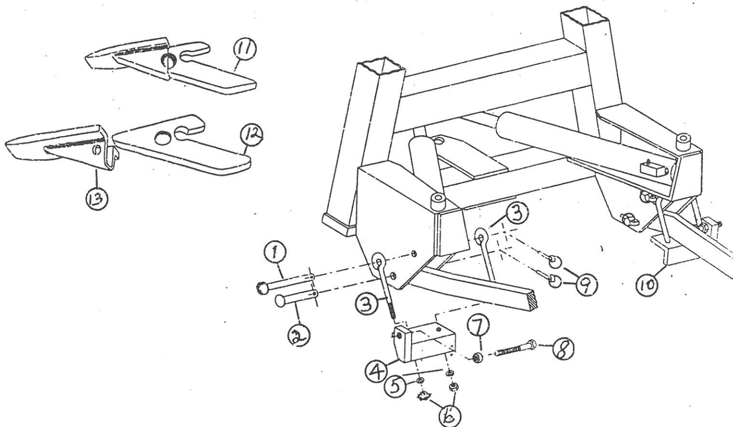
LOWER LINK LOCKS AND BUCKET TEETH
