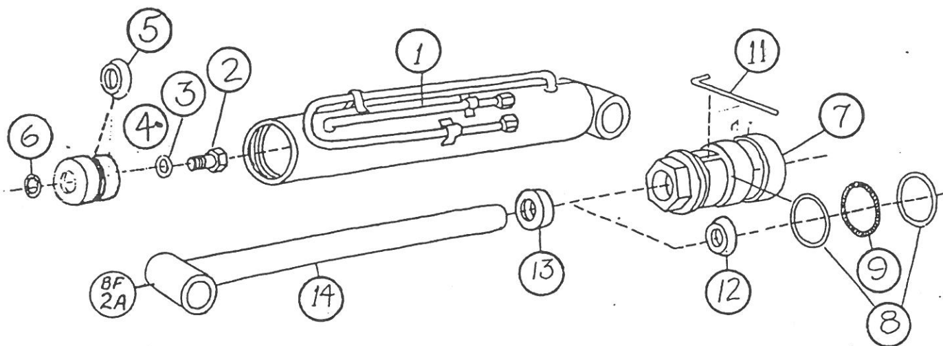
BCY10948, 2-1/2" x 13" FOLDING AND GULL WING STABILIZER CYLINDER
