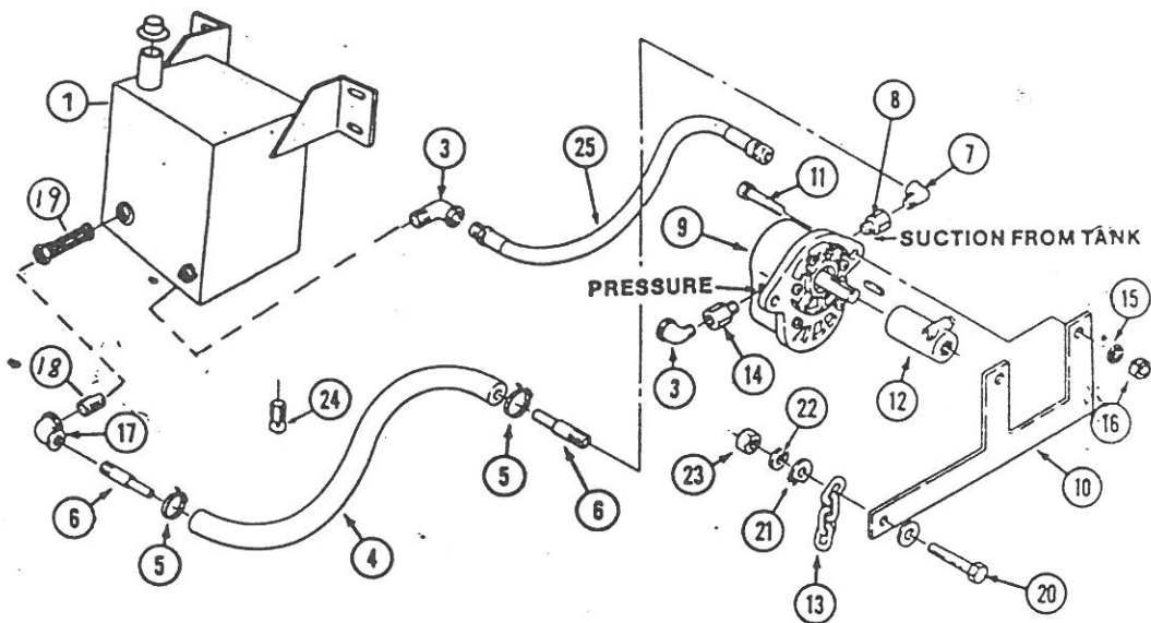
BCP 10360-1000RPM-PTO INDEPENDENT HYDRAULIC PUMP SYSTEM
