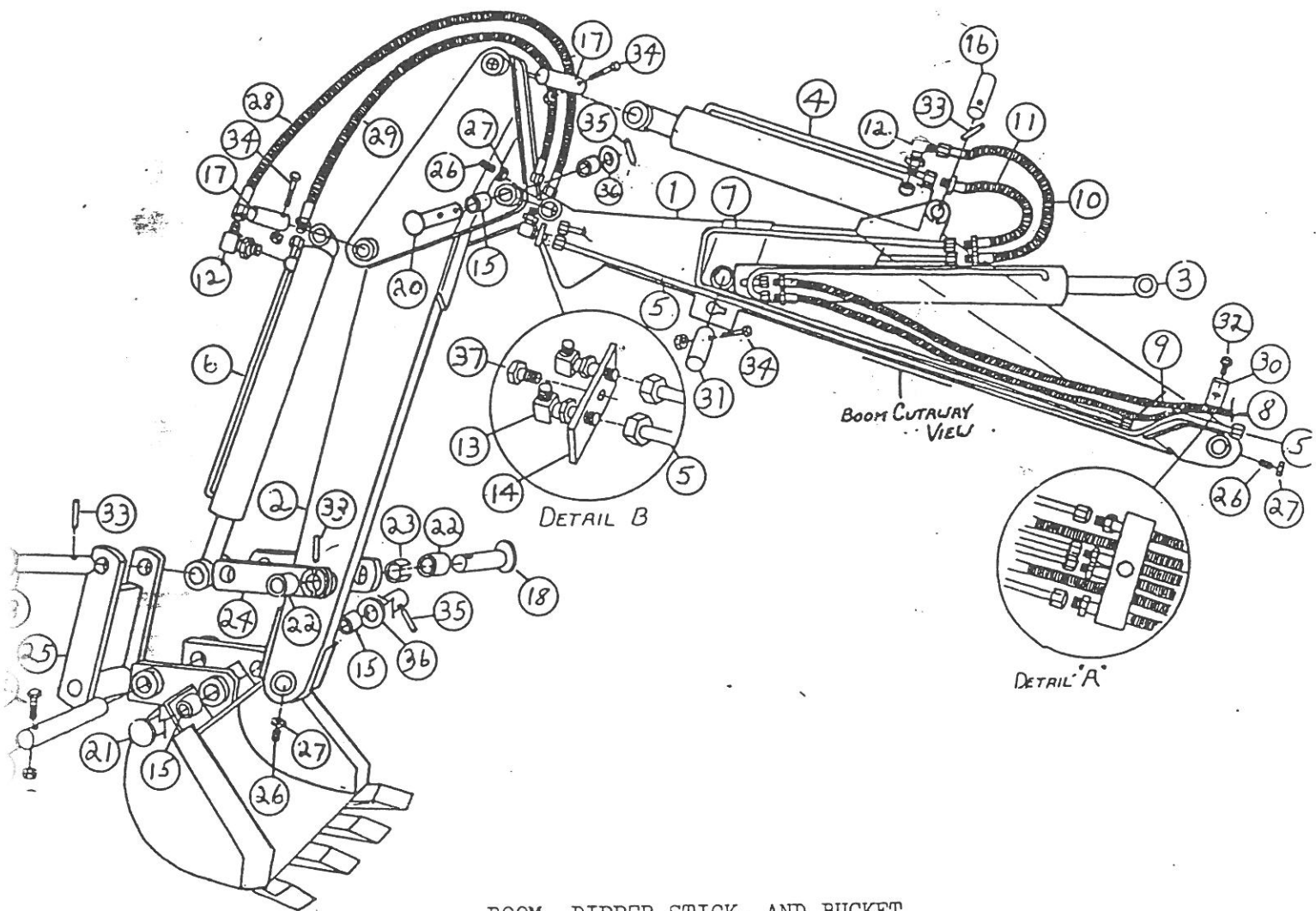
BOOM, DIPPER STICK, AND BUCKET
