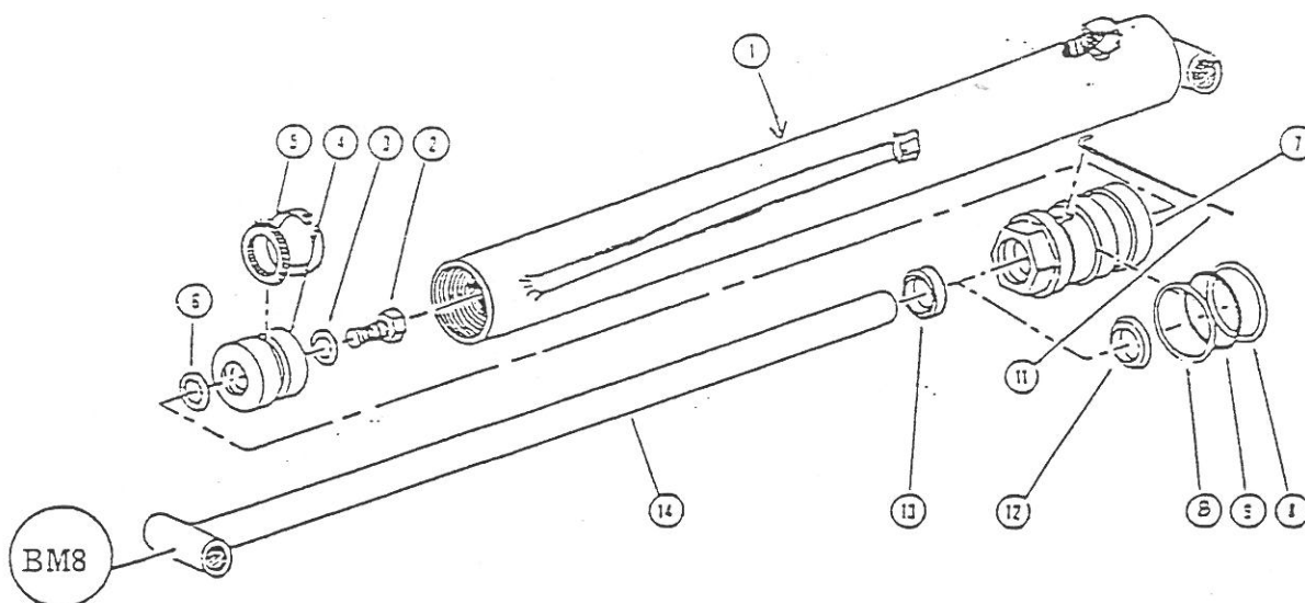
BCY 12686 Bucket Cylinder 2½" x 14"
