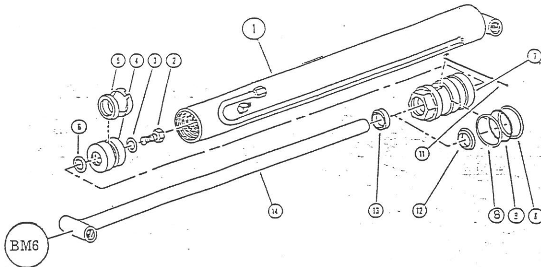
BCY 12684 BOOM Cylinder 2½" x 20"
