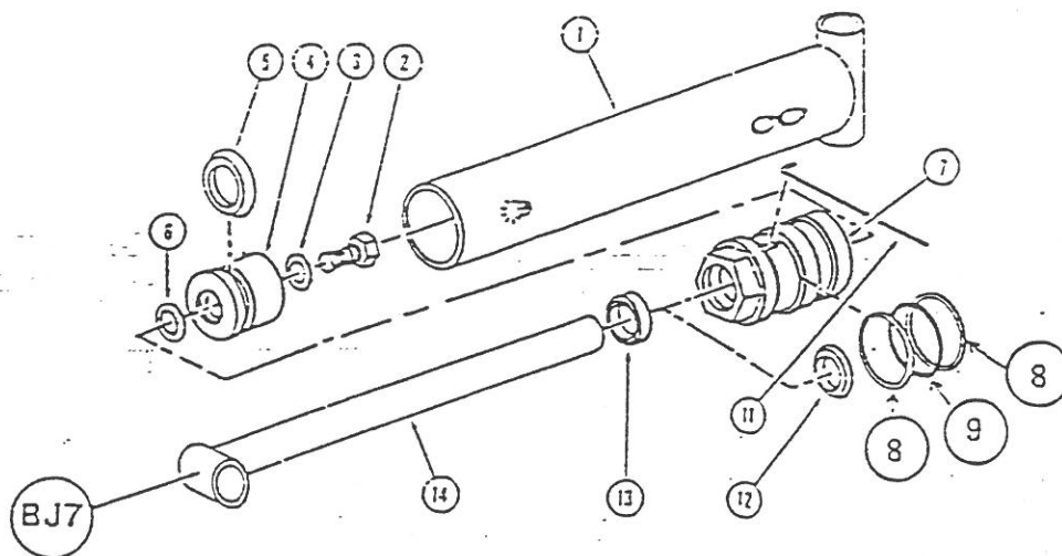
BCY 302 SWING Cylinder 2-1/2" x 10"
