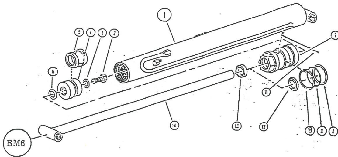
BCY 12684 BOOM Cylinder 2½" x 20"
