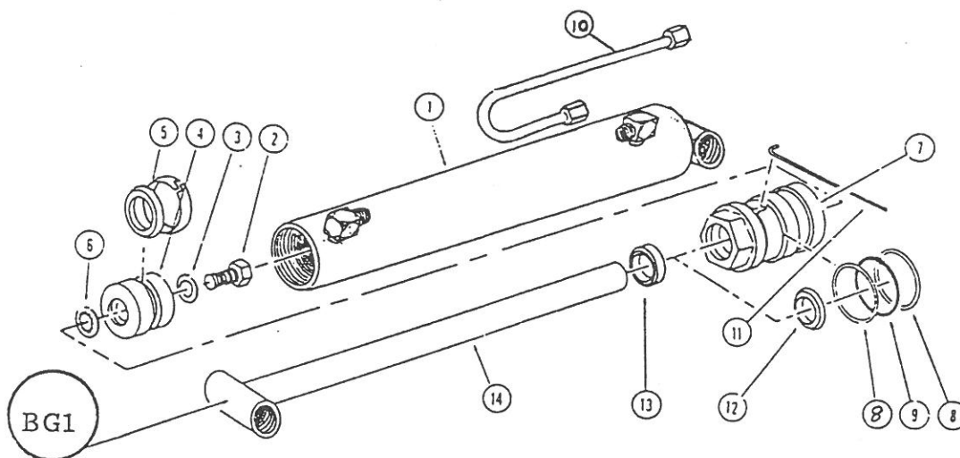
BCY12529 BOOM CYLINDER 2-1/2" X 14"
