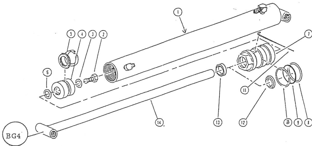
BCY12538 STABILIZER CYLINDER 2-1/2" X 8"
