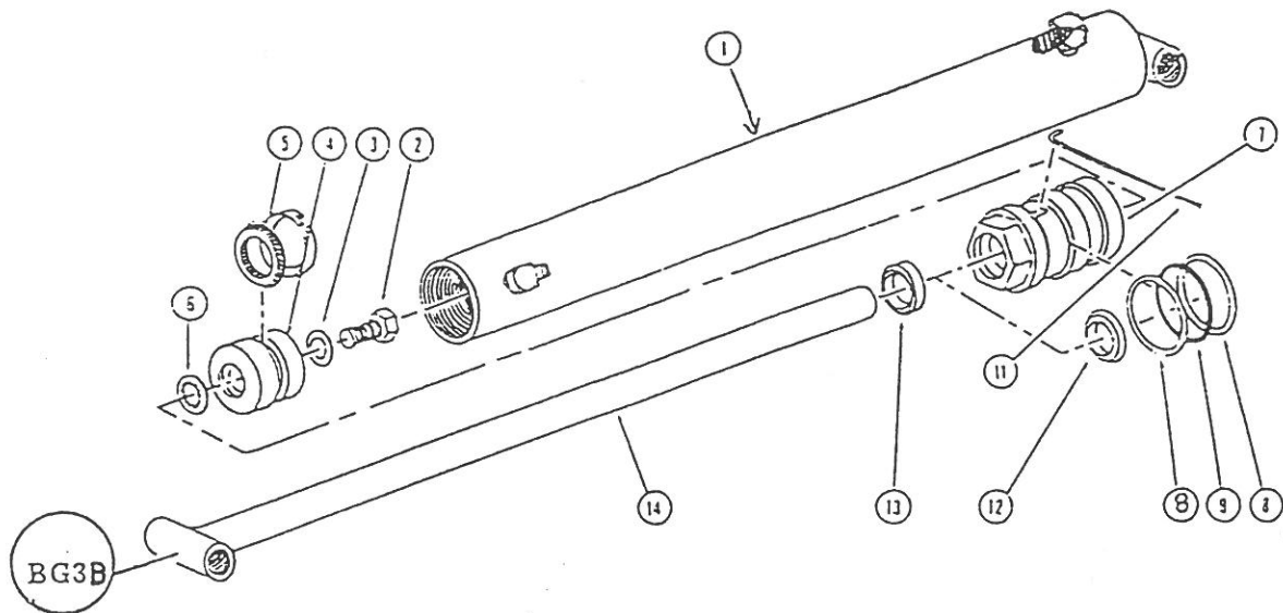
BCY13081 Bucket Cylinder 2" x 12"
