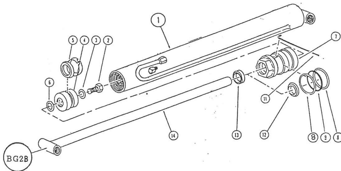
BCY13080 Dipper Stick Cylinder 2-1/3" x 10"
