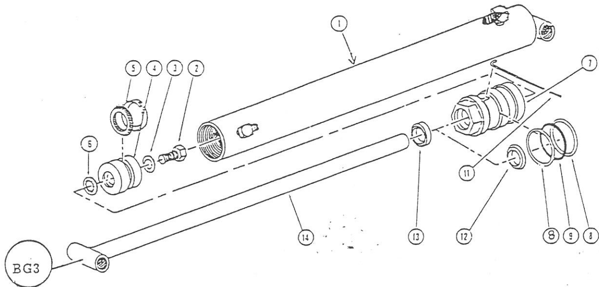
BCY12531 BUCKET CYLINDER 2" X 12"
