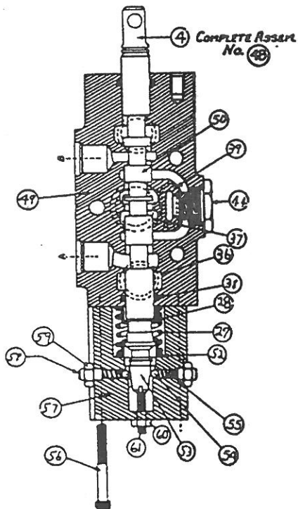
DIRECT RELIEF VALVE CARTRIDGE W/EXTERNAL ADJUSTMENT CODE LETTER 'F' 785056
